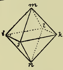
III. Octohedron
